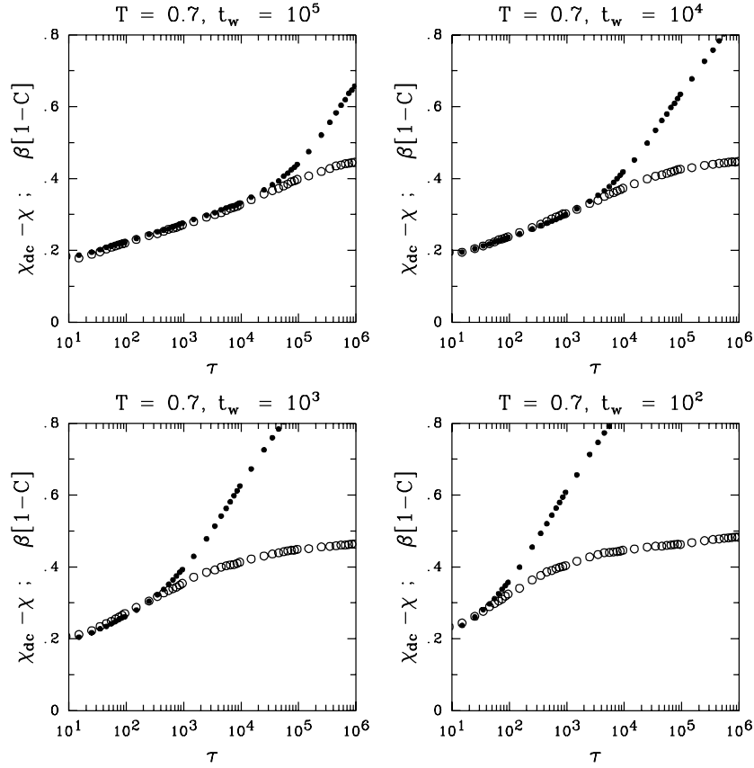
Figure 22. Zero-field cooled IRF \chi_{\text{ZFC}}(t, t_w) = M_{\text{ZFC}}(t, t_w)/h = \chi_{dc} - \chi_{\text{FC}}(t, t_w) (empty circles) in the 3D EA model plotted as a function of the time t \equiv \tau for different values of t_w at T = 0.7 . For times t \equiv \tau > t_w deviations from the FD relation \chi_{\text{ZFC}}(t, t_w) = \beta(1 - C(t, t_w)) (full circles) are noticeable. From [247].
